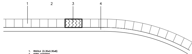
DETALL POU EMBORNAL 1/50
